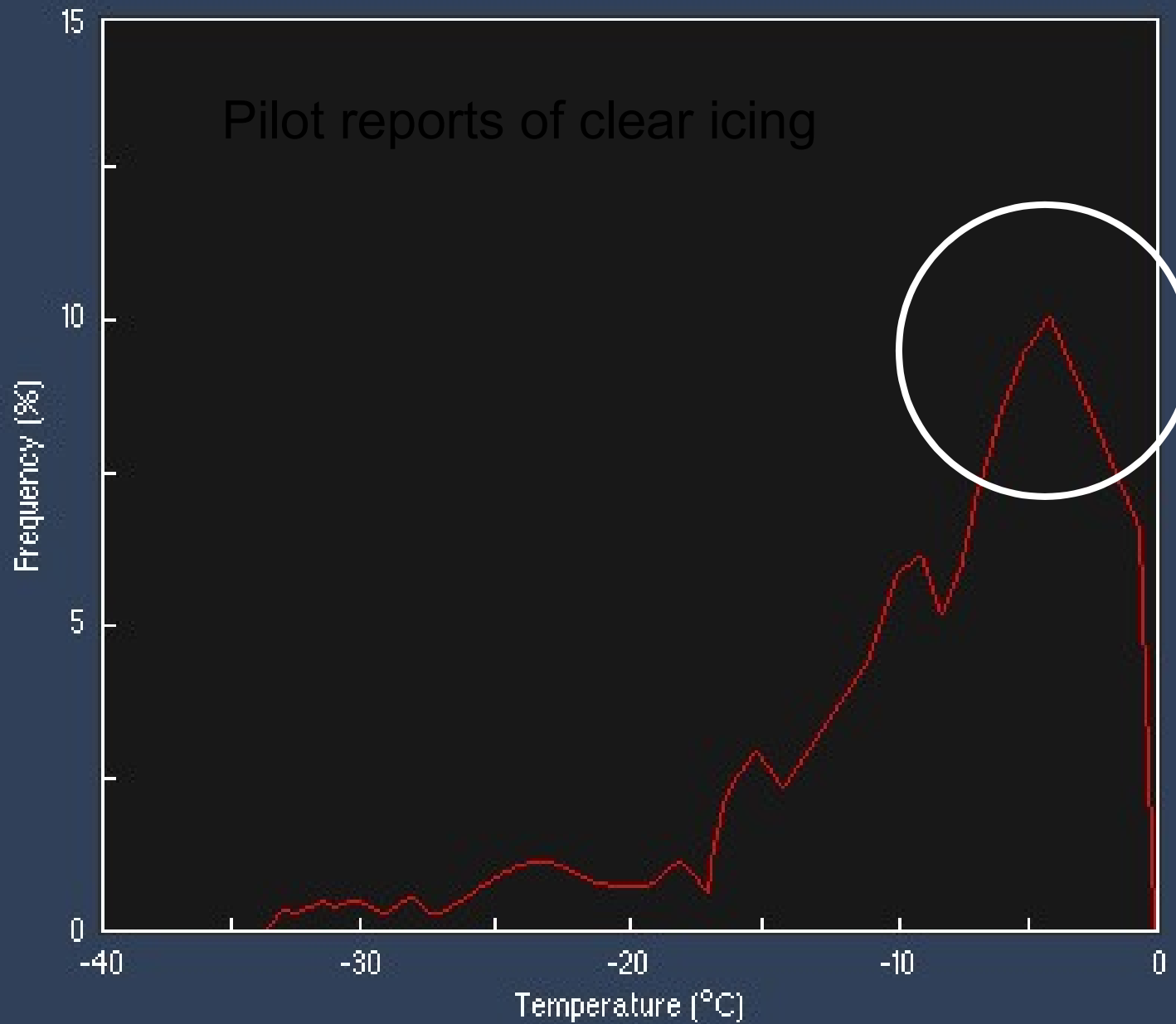
Clear Icing PIREP Frequency vs Temperature
