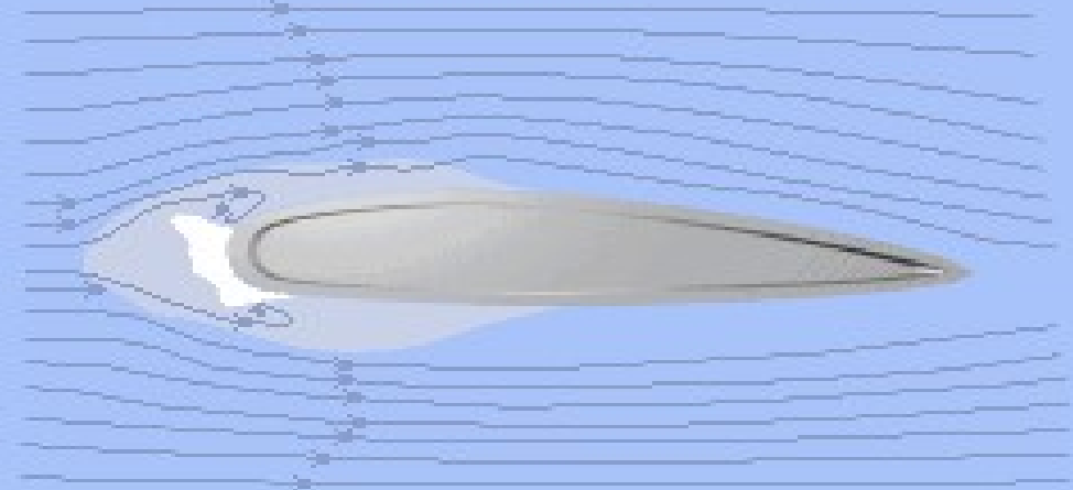
Flow Disruption from Clear or Mixed Ice
