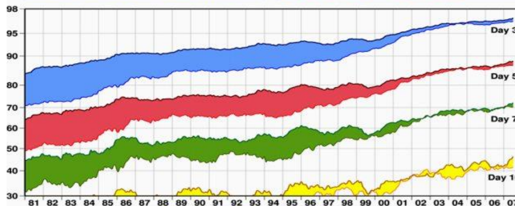
Anomaly correlation (%) of 500hPa height forecasts
