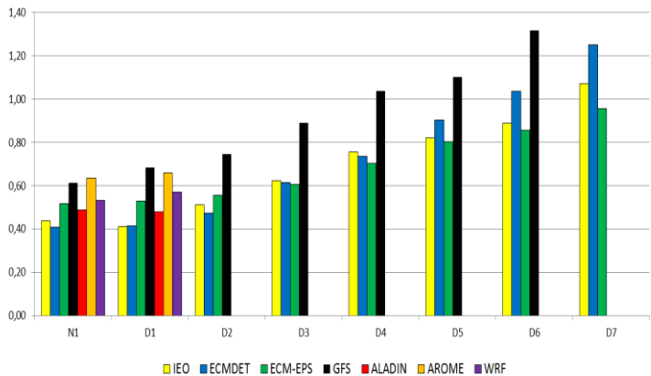
Total cloudiness, mean absolute error - 2018
